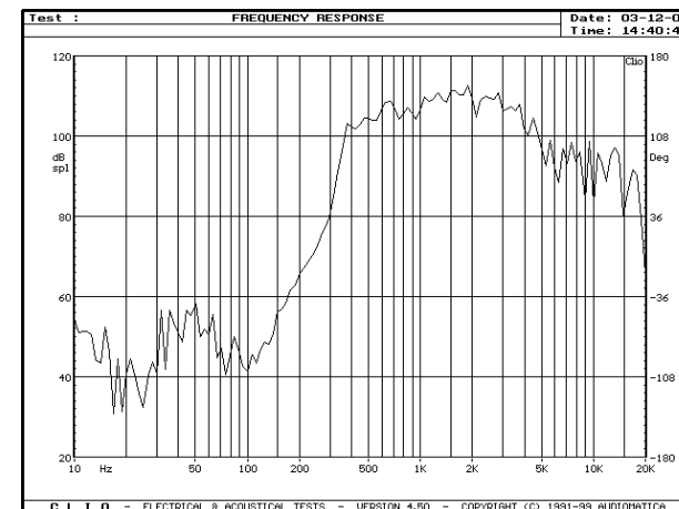
FREQUENCY RESPONSE
